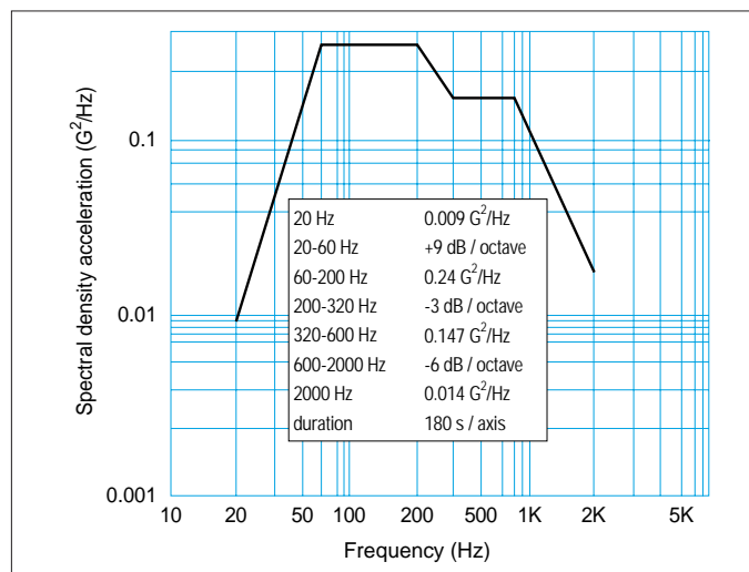
Diagram 2: Vibration
