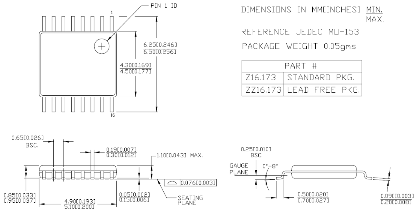
Figure 11. 16-Pin TSSOP 4.40 mm Body Z16.173
