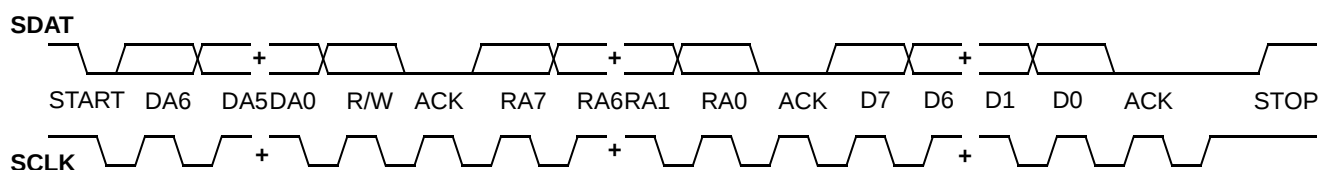
Figure 6. Frame Format (Device Address, \overline{R/W} , Register Address, Register Data
