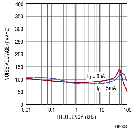
1.2V Output Voltage Noise Spectrum
