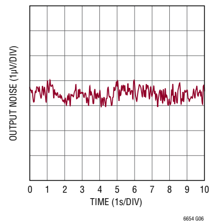
1.25V Output Noise 0.1Hz to 10Hz
