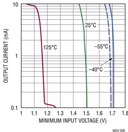
1.25V Minimum Input Voltage (Sinking)
