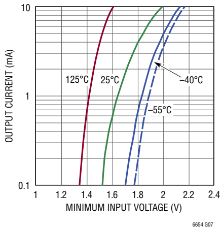
1.25V Minimum Input Voltage (Sourcing)
