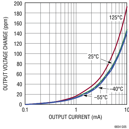
1.25V Minimum Input Voltage (Sinking)
