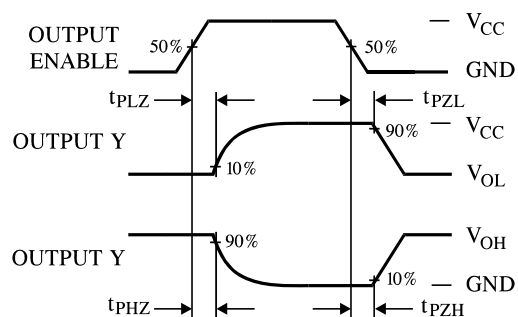
Figure 2. Switching Waveforms
