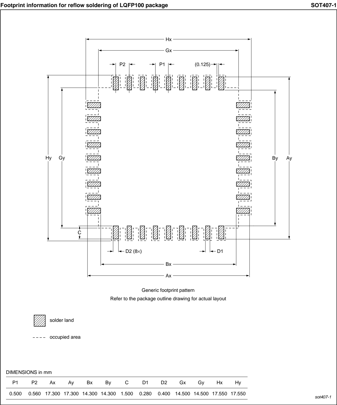
Fig 47. Reflow soldering for the LQFP100 package
