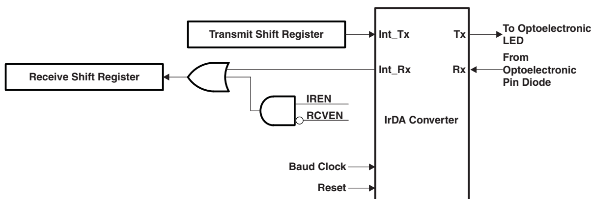
Figure 25. IrDA Mode
