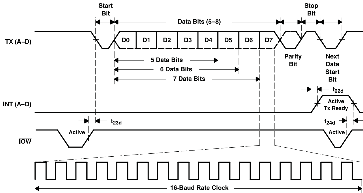
Figure 19. Transmit Timing
