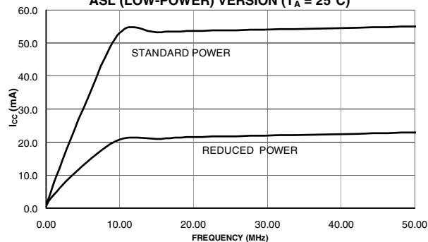
SUPPLY CURRENT VS. FREQUENCY ASL (LOW-POWER) VERSION ( T_A = 25^\circ\text{C} )
