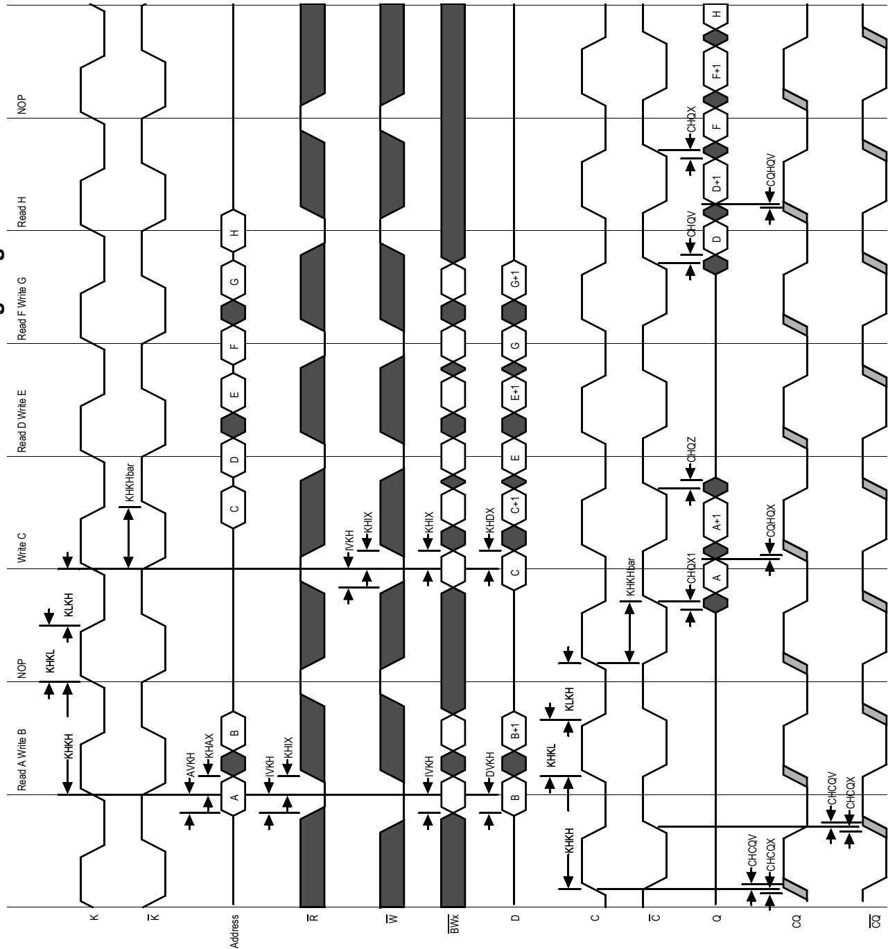
C and \overline{C} Controlled Read-Write-Read Timing Diagram
