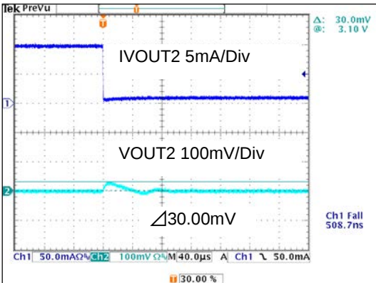
Figure 28. Load Response(Fall) (VBAT=3.6V,Cout=4.7 μ F,Ta=25°C,Iout=10mA→1mA,Tf=0.5 μ s)
