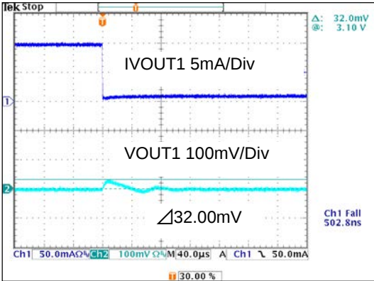
Figure 26. Load Response(Fall) (VBAT=3.6V,Cout=4.7 μ F,Ta=25°C,Iout=10mA→1mA,Tf=0.5 μ s)
