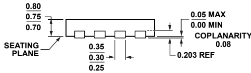
COMPLIANT TO JEDEC STANDARDS MO-229-WEEC-2 Figure 39. 8-Lead Lead Frame Chip Scale Package [LFCSF_WD] 3 mm x 3 mm Body, Very Very Thin, Dual Lead (CP-8-15) Dimensions shown in millimeters
