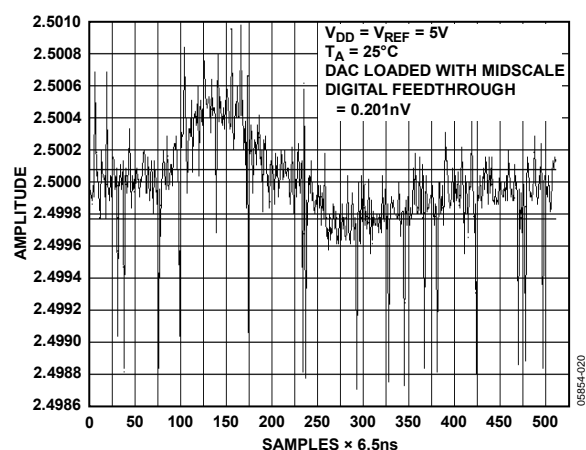
Figure 18. Digital Feedthrough
