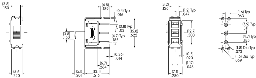
Actuator in LEFT Position
