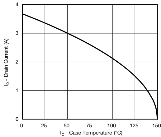
Current Derating*
