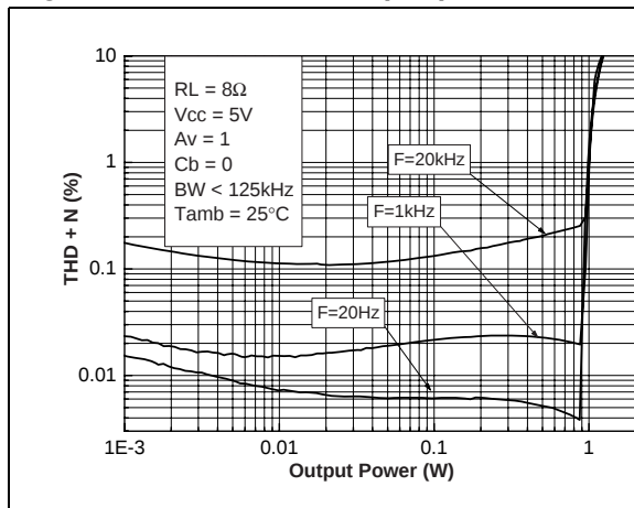
Figure 57. THD+N vs. output power
