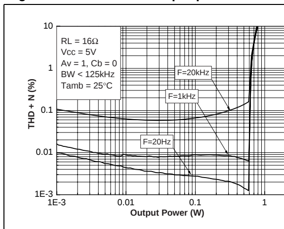
Figure 59. THD+N vs. output power
