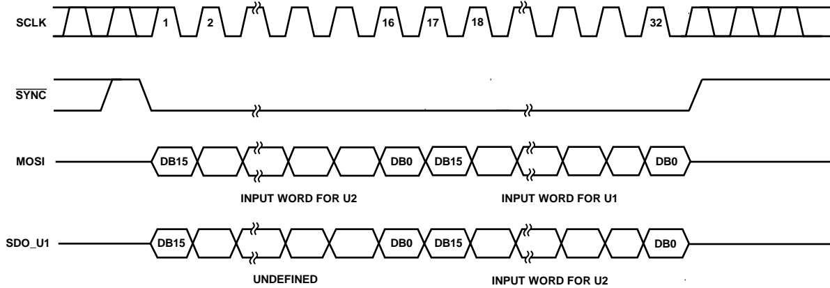
Figure 45. Daisy-Chain Diagram
