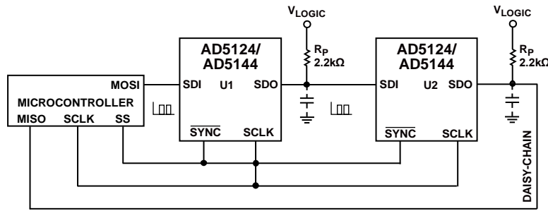
Figure 44. Daisy-Chain Configuration
