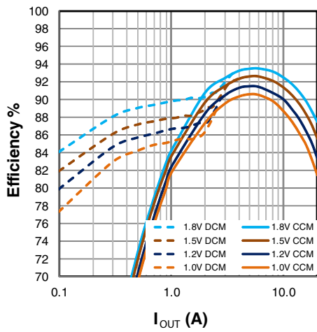
Figure 19: Efficiency, V_{IN}=5\text{V}
