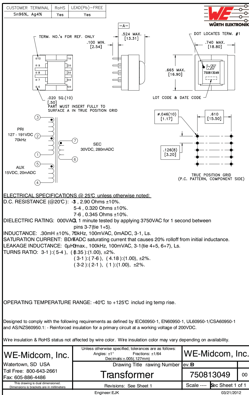
Figure 28. Transformer Specification
