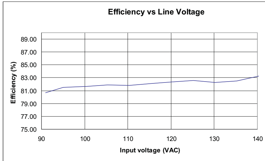
Figure 3. LM3447-A19-120VEVM Efficiency
