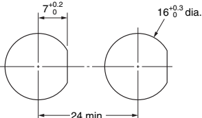
Panel Cutouts
