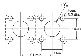
Panel Cutouts
