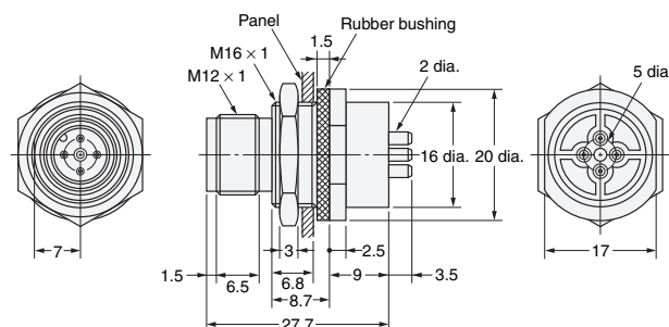
PCB-mounting Dimensions
