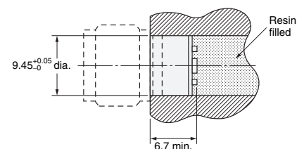
Mounted Dimensions
