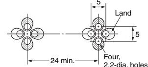
PCB-mounting Dimensions
