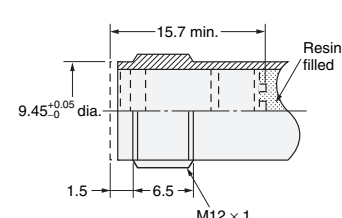
Mounted Dimensions
