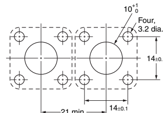
Panel Cutouts
