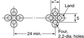
PCB-mounting Dimensions
