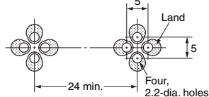
PCB-mounting Dimensions
