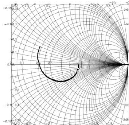
FIGURE 12. SMITH CHART OF S22
