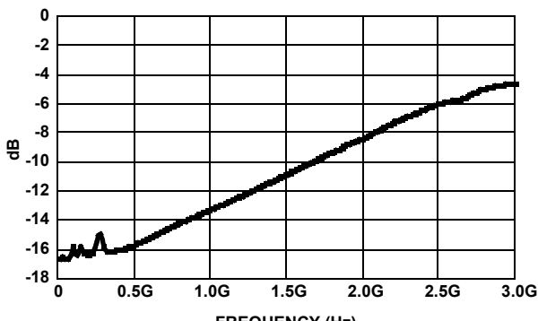
FIGURE 11. |S22| vs FREQUENCY
