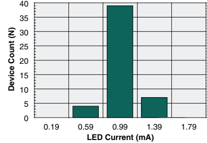
Typical I F for Switch Dropout (N=50, I F =5mA, I L =100mA DC )
