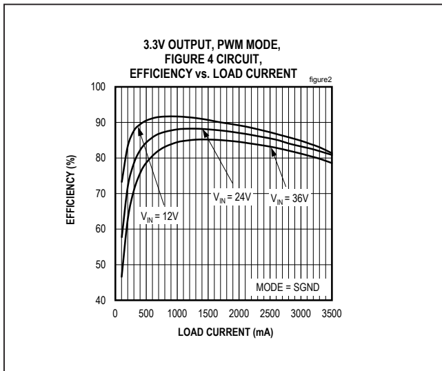
Figure 2. MAX17544 3.3V Output Efficiency (PWM Mode)
