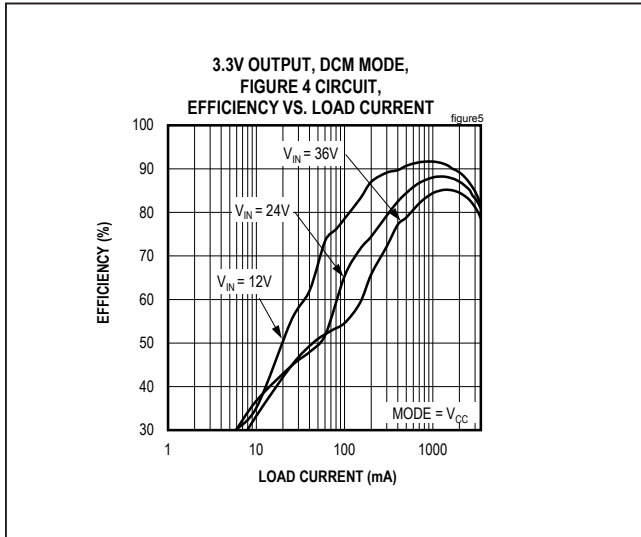
Figure 5. MAX17544 3.3V Output Efficiency (DCM Mode)
