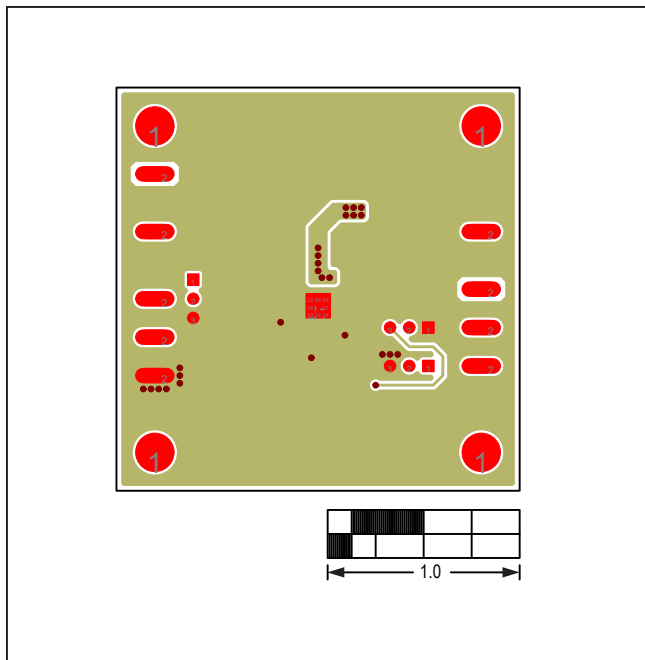
Figure 16. MAX17544 3.3V Output EV Kit PCB Layout—Solder Side
