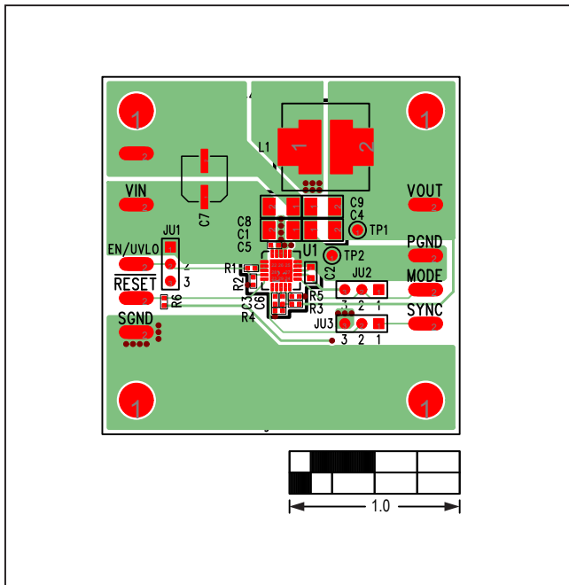
Figure 13. MAX17544 3.3V Output EV Kit Component Side PCB layout
