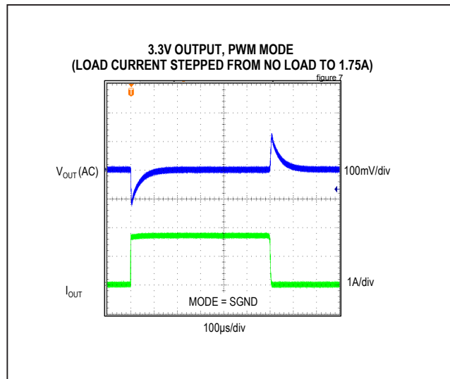
Figure 7. MAX17544 3.3V Output, No Load to 1.75A Load Transient (PWM Mode)
