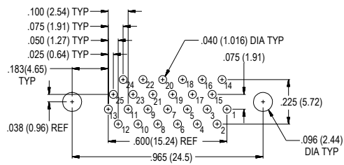
25 PIN MWDM-25PCBS
