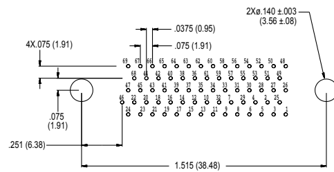
69 PIN MWDM-69PCBS
