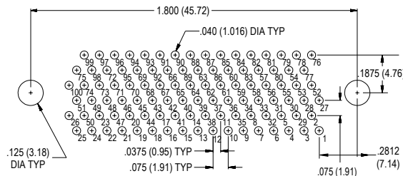
100 PIN MWDM-100PCBS
