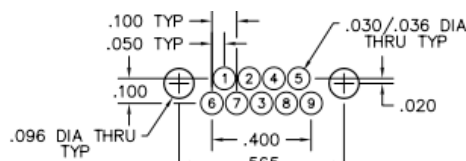
PC BOARD LAYOUT COMPONENT SIDE
