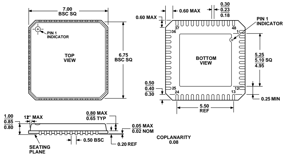
Figure 27. 48-Lead Lead Frame Chip Scale Package [LFCSP] 7 mm x 7 mm Body (CP-48) Dimensions shown in millimeters
