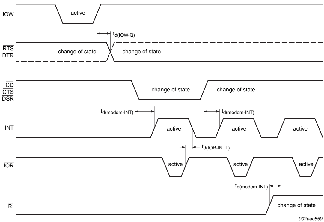
Fig 9. Modem input/output timing
