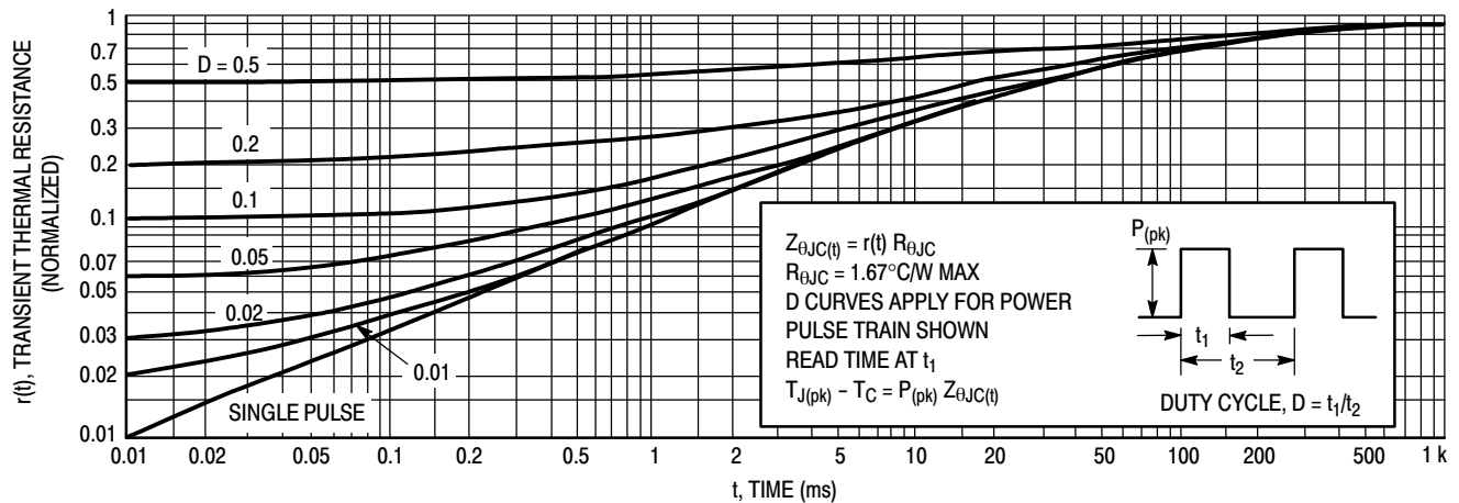
Figure 10. Typical Thermal Response [Z_{\theta\text{JC}}(t)]
