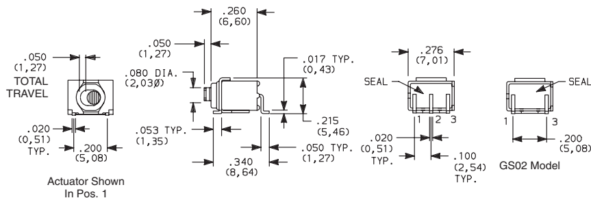
SMT GS01MSABE Horizontal Actuation SPDT
