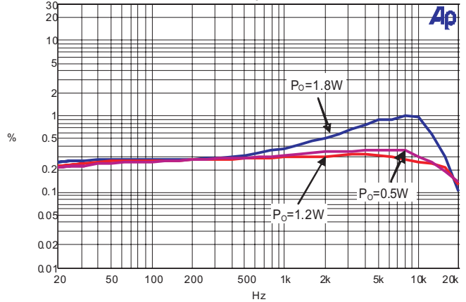
THD+N vs Frequency V_{DD}=5\text{V} , R_L=4\Omega , C_{IN}=1\mu\text{F} , Gain=23dB
