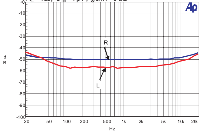
PSSR vs Frequency Input ac-ground, V_{DD}=5\text{V} 200mVpp, R_L=4\Omega , C_{IN}=1\mu\text{F} , gain=5dB
