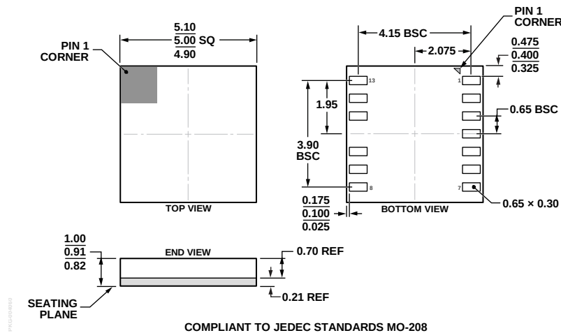
Figure 23. 13-Terminal Land Grid Array [LGA] (CC-13-1) Dimensions shown in millimeters
