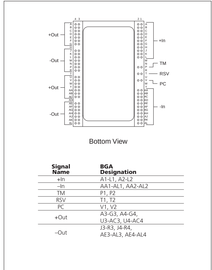
Figure 14—BCM BGA configuration
