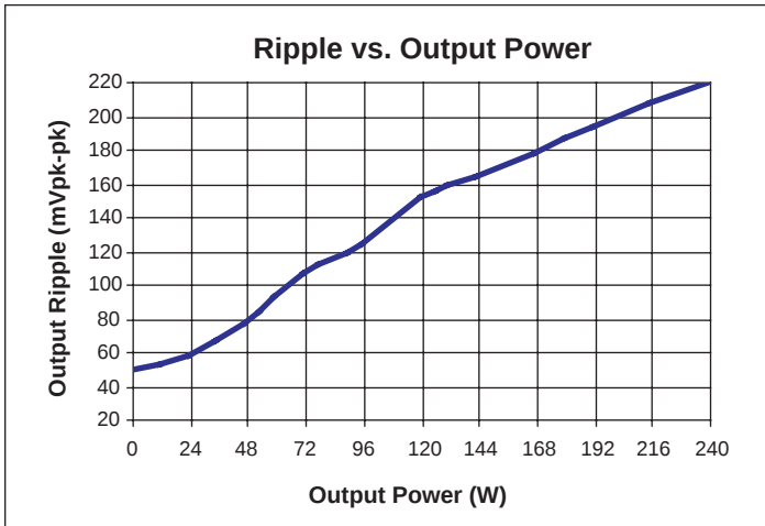
Figure 9 — Output voltage ripple vs. output power at 48 Vin line without any external bypass capacitor.
