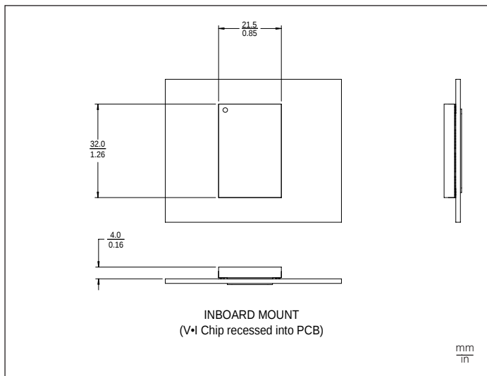
Figure 19—Inboard mounting – package K
