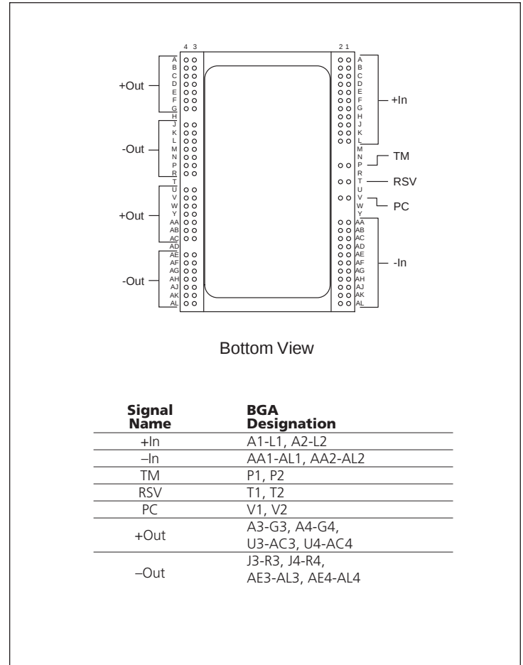
Figure 14—BCM BGA configuration
