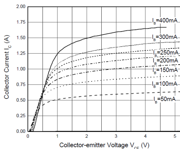
Static Characteristics
