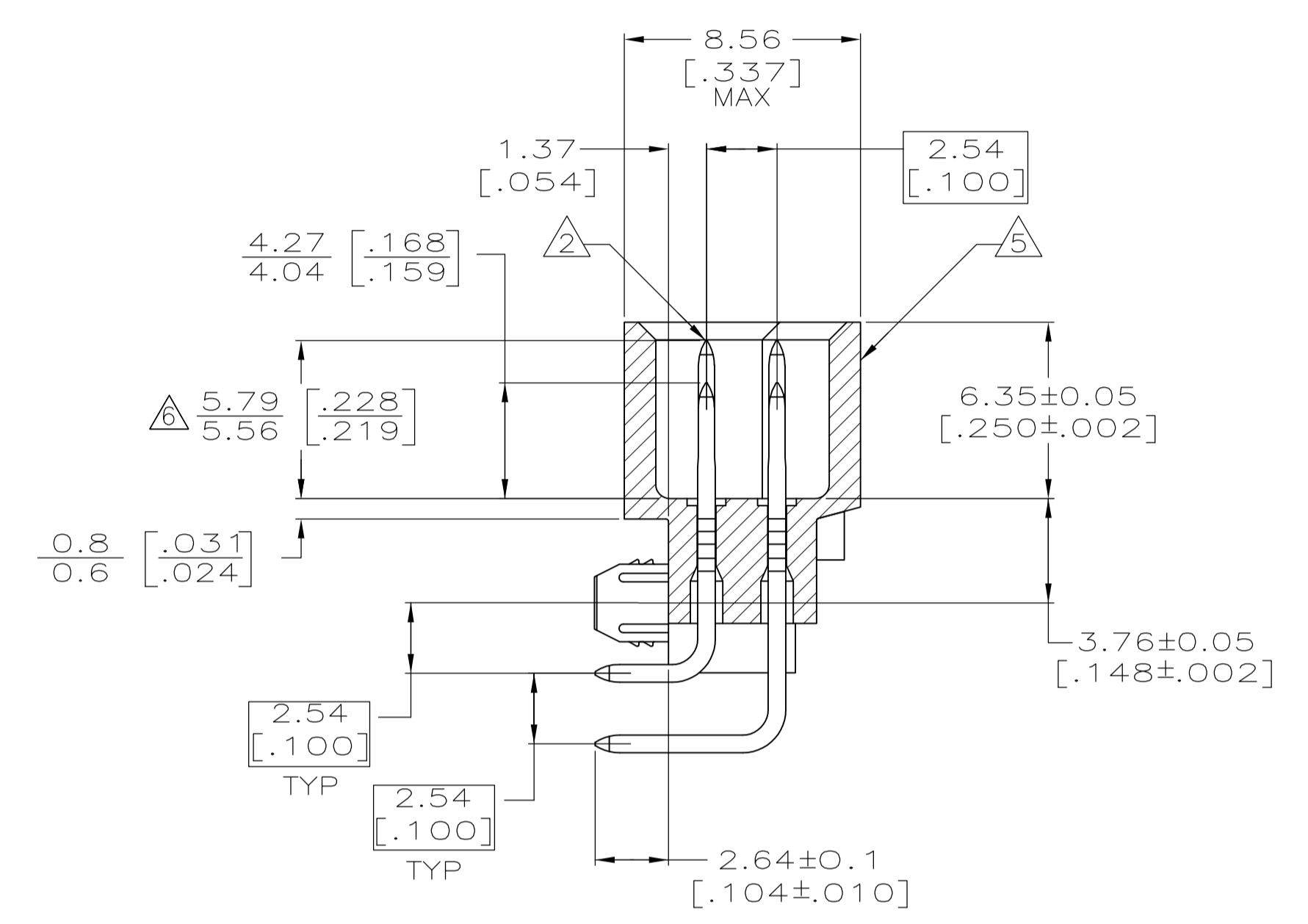
SECTION Z-Z
