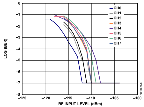
Figure 5. Sensitivity Plot
