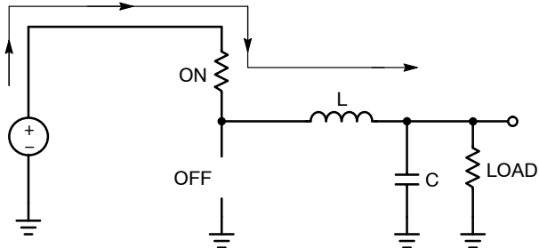
Figure 17. Buck Topology Inductor Current During t_0 and t_1
