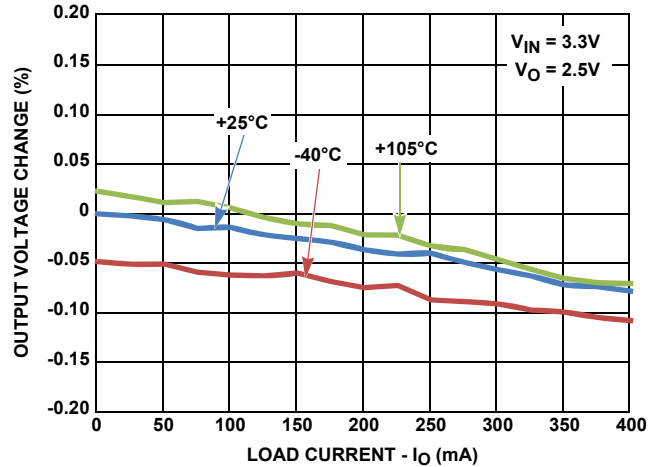
FIGURE 3. LOAD REGULATION
