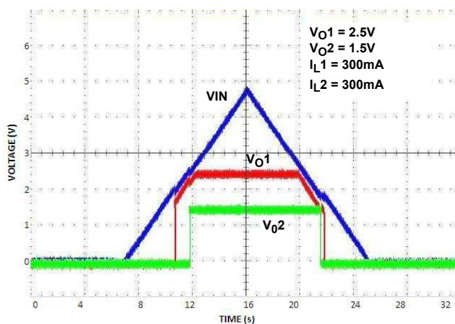
FIGURE 10. POWER-UP/POWER-DOWN
