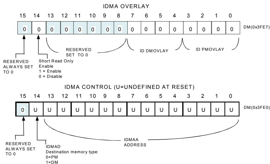
Figure 9. IDMA Control/OVLAY Registers
