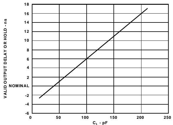
Figure 18. Typical Output Valid Delay or Hold vs. Load Capacitance, CL (at Maximum Ambient Operating Temperature)
