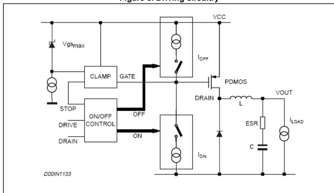
Figure 8. Driving circuitry
