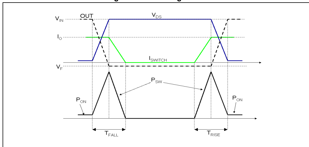
Figure 14. Switching losses
