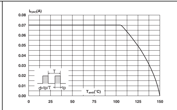
Figure 2. Average forward current I_{F(AV)} versus ambient temperature T_{amb} ( \delta = 1 )
