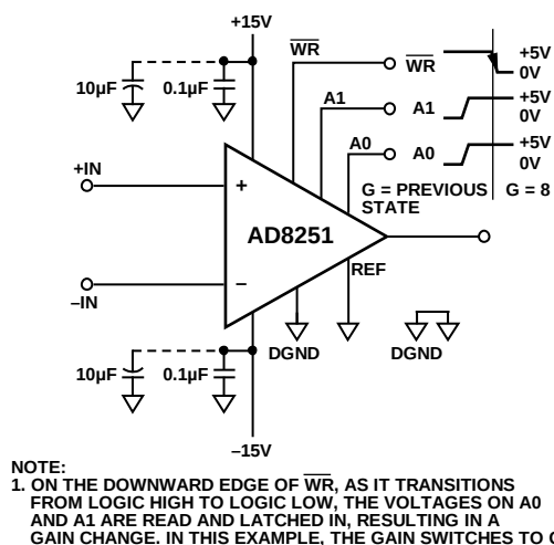
Figure 53. Latched Gain Mode, G = 8
