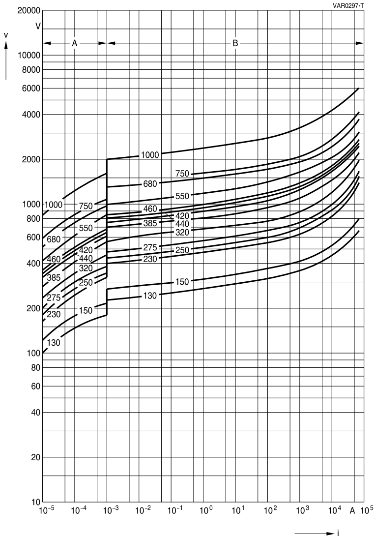
SIOV-B60K130 ... K1000
