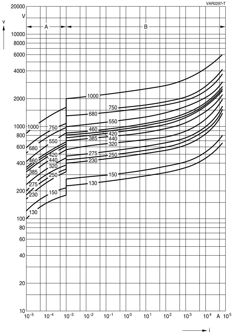
SIOV-B60K130 ... K1000
