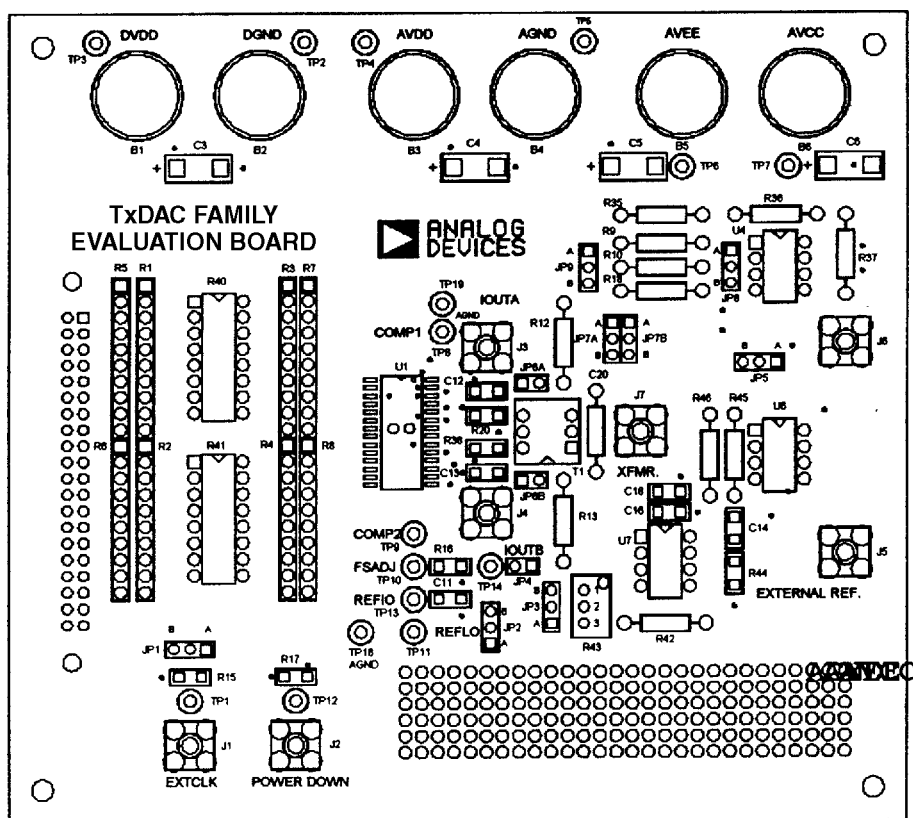
Figure 60. Silkscreen Layer—Top
